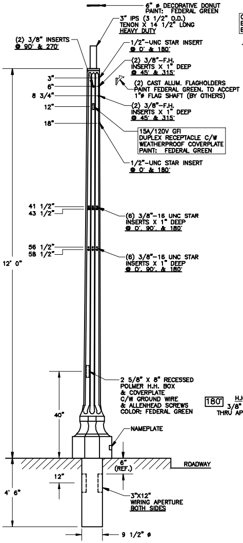
SINGLE HEAD CONCRETE POLE STREET LIGHT - 400W METAL HALIDE NOT TO SCALE PLATE 2005
